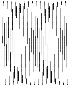
Figure 1 Shape of \phi_\alpha for \alpha large, n = 1 .
