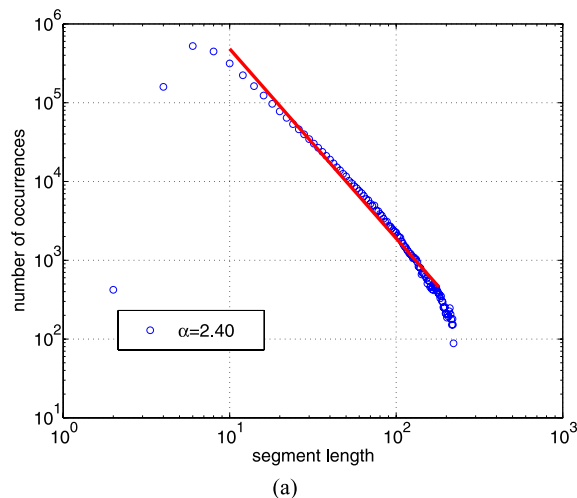
Fig. 3 Empirical distributions of approximately straight contour segment length |L| . (a) The marginal distribution of |L| on a log-log scale. It closely follows a power law with \alpha = 2.40 , in direct contradiction
