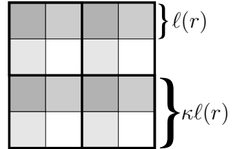
Figure 2: Illustration of a coloring scheme ( \kappa = 2 ).
