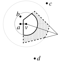
Figure 1: \mathcal{M} = \{a, b, c, d, v\} . \text{NN}_{\mathcal{M}}(v) = |va| . Thick solid and dashed boundaries show \text{Vor}_{\mathcal{M}}^{\rho}(v) and \text{Vor}_{\mathcal{M}}^{\beta}(v) , where \rho = 2 and \beta = 4 . The \rho -clipped Voronoi neighbors of v are a and b . Shaded region is the (\rho, \beta) picking region of v .
