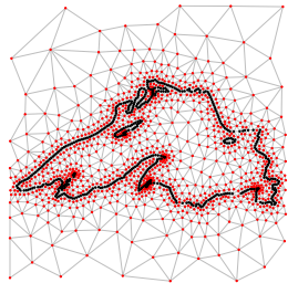
Figure 8: A model of Lake Superior meshed by StableWS .
