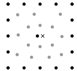
Figure 6: Inserting x creates \Omega(\log \Delta) fresh Steiner vertices.
