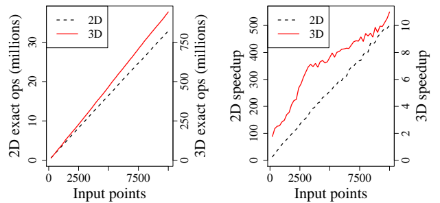
Figure 7: Left: cost of StableWS on random inputs. Right: speedup of PropagateWS one unit changes relative to StableWS from scratch.
